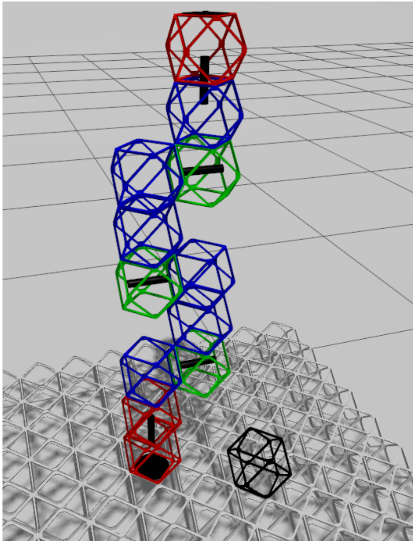
Figure 5.2: Robot structure in Gazebo simulation environment
