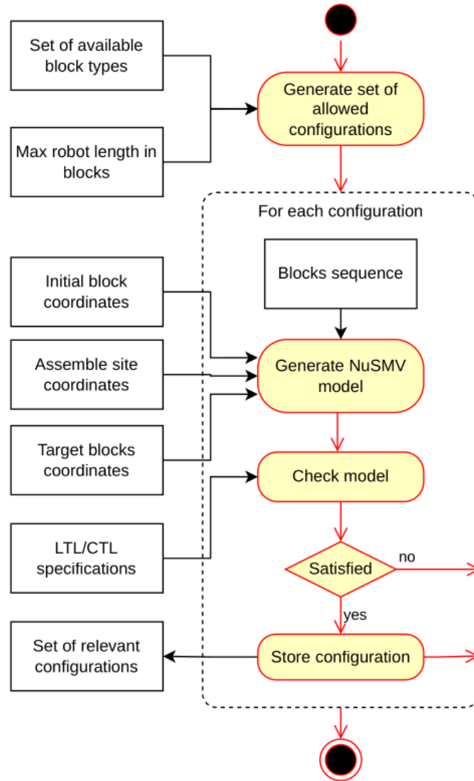
Figure 5.8: Activity diagram of searching for relevant configurations
